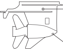
Gear oil level plug
