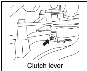
Clutch lever
